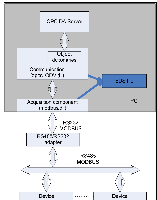
Figure 2. EDS interpretation
