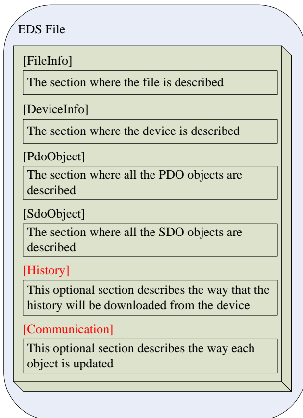
Figure 1. Electronic device description file
