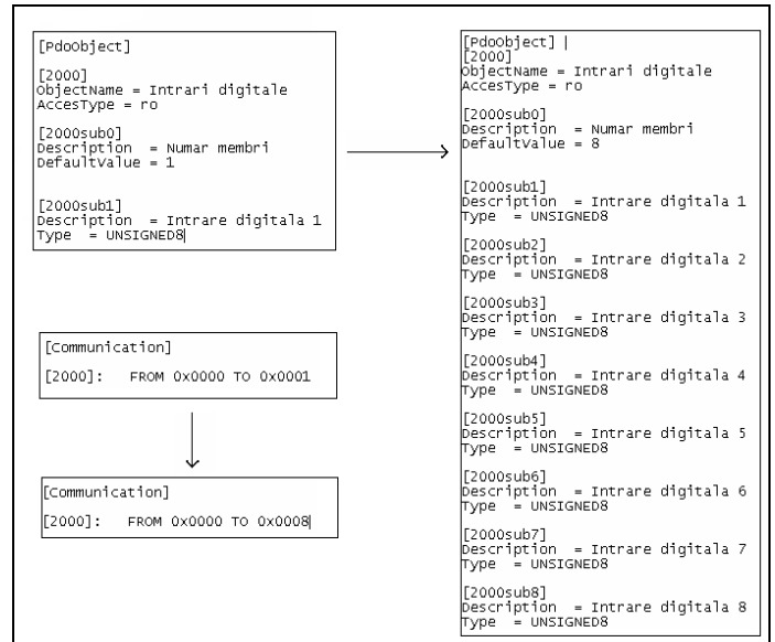
Figure 4. EDS file example
